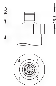
M12x1
